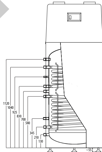
Basic 270 with 2 coils
